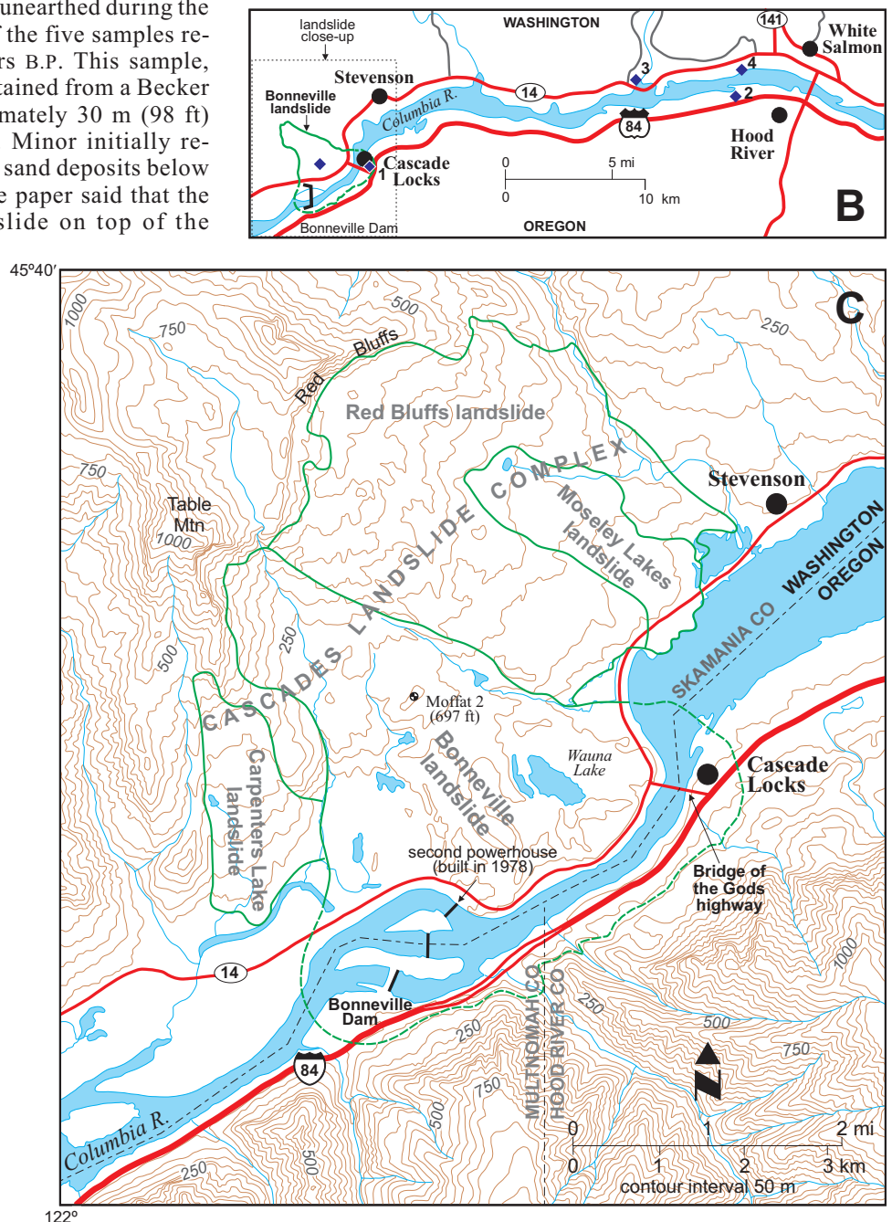
Figure 2. A. Location of study area within Washington State. B. Study area with sampling site locations of the four reference datasets (numbered diamonds) and sampling site on the landslide deposit. C. Close-up showing approximate boundary of the Bonneville landslide within the Cascades landslide complex; dashed where approximate maximum extent inferred (after Schuster and Pringle, in press).
